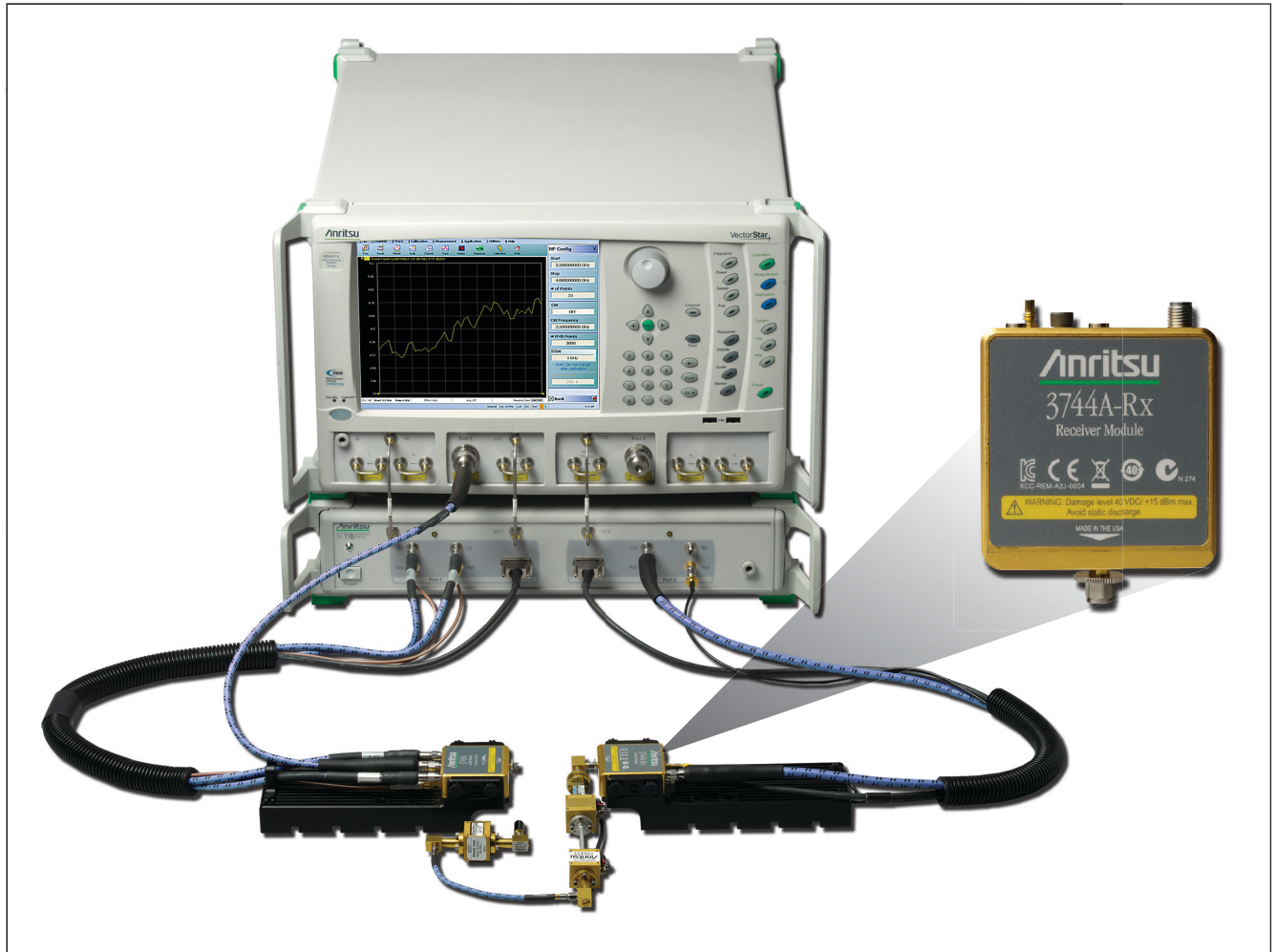
ME7838A with 3744A-Rx Receiver Module
