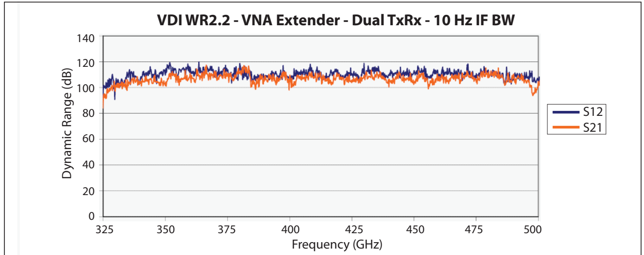
Dynamic Range Plot of VDI WR2.2 Module – 10 Hz IFBW
