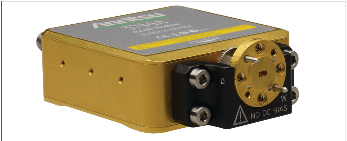
3744A-EE/3744A-EW Millimeter-Wave Module with Waveguide Adapter
